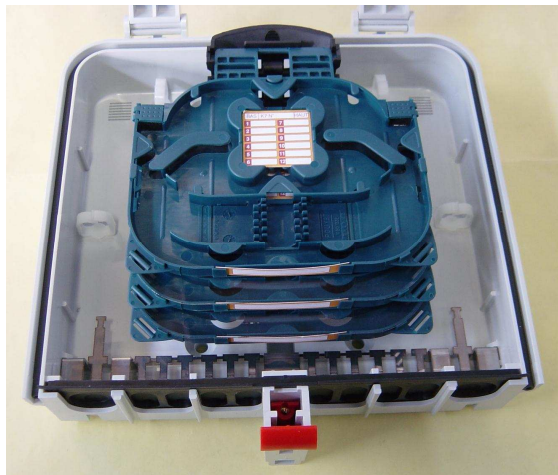
Distribution Box PBO Size 1
